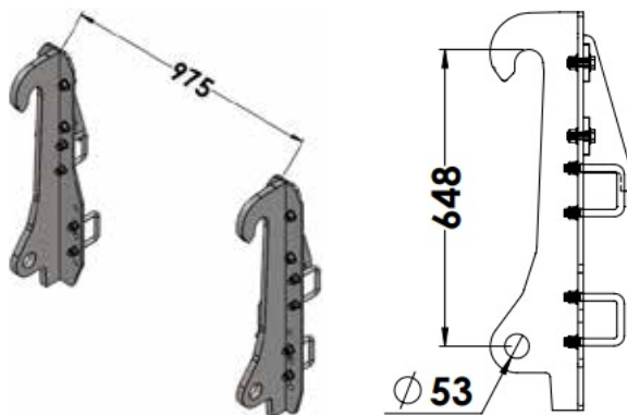
* LBVOLA - Loader Brackets Bolt on Volvo
