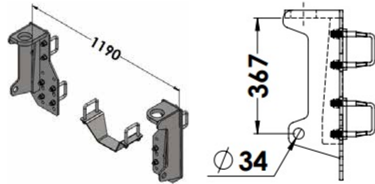
* LBMTBA - Loader Brackets Bolt on Matbro
