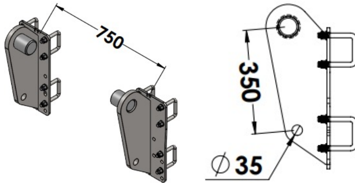
* LBMTUA - Loader Brackets Bolt on Manitou
