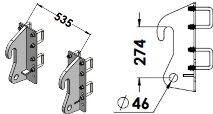
* LBCPTA - Loader Brackets Bolt on JCB Compact
