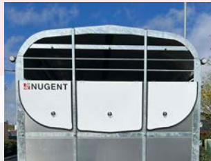
Nugent's unique trio of fold down front panels allow farmers to control the level of air flow through the trailer. This reduces drag to provide for a better towing trailer, while significantly decreasing fuel consumption.
